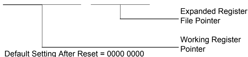
Figure 14. Register Pointer
