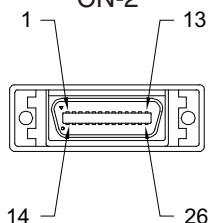
MDR 26 Position Plug Frame Grabber End CN-2
