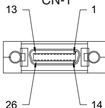
MDR 26 Position Receptacle Camera End CN-1
