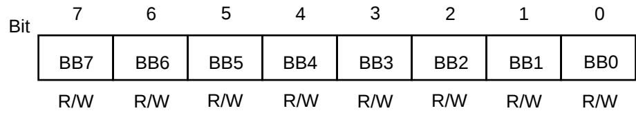
Figure 80. MMU Bank Base Register (BBR: I/O Address = 39H)
