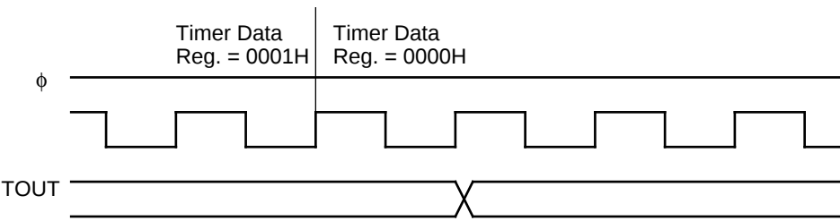
Figure 6. Timer Output Timing
