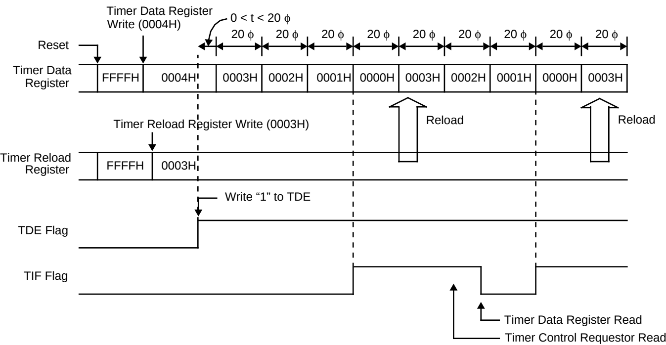
Figure 5. Timer Initialization, Count Down, and Reload Timing
