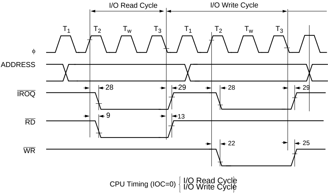
Figure 22. CPU Timing (I/O = 0) (I/O Read Cycle, I/O Write Cycle)
