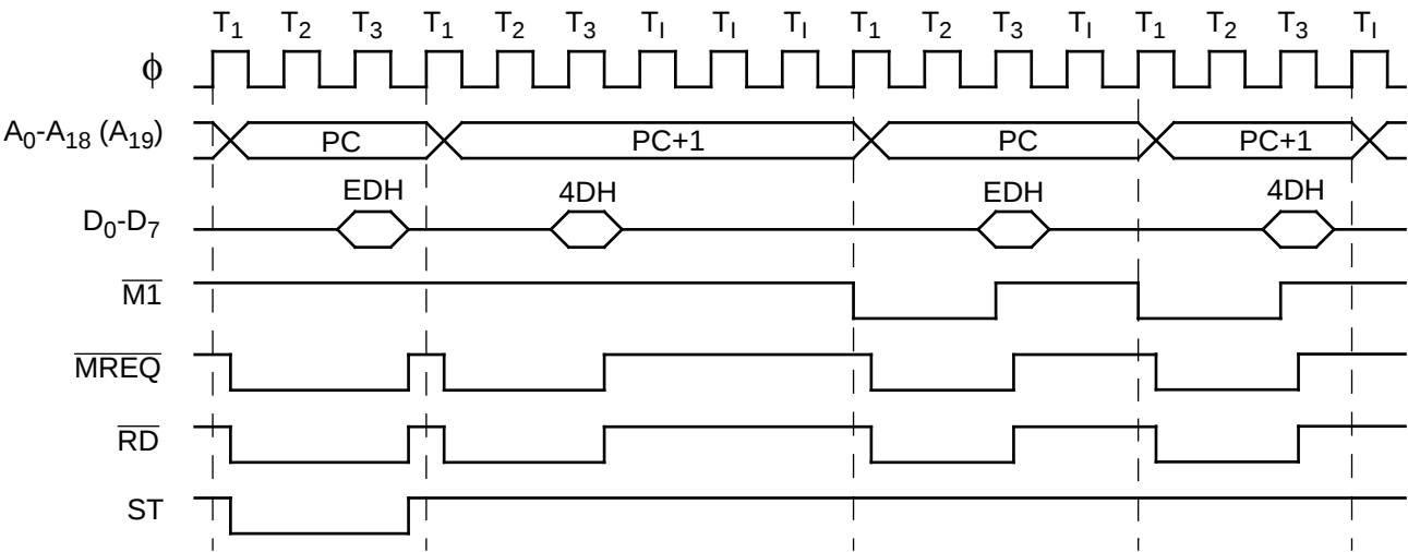
Figure 83. RETI Instruction Sequence with M1E=0
