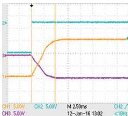
Typical Start-Up Wave Form
