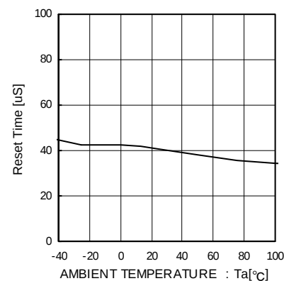
Fig. 12 Power-on Reset Time vs Temperature
