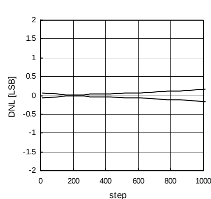
Fig. 18 Differential Linearity Error
