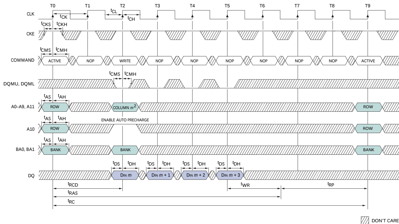
Figure 51: Write – With Auto Precharge
