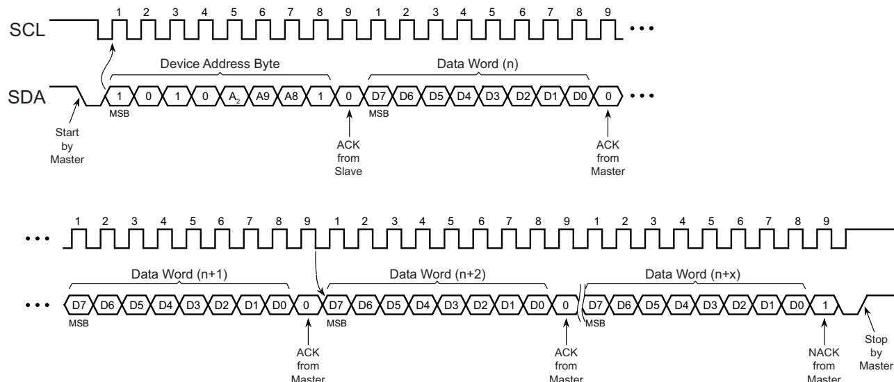
Figure 6-3. Sequential Read
