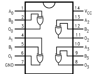
Figure 1. Connection Diagram
