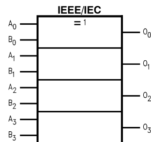
Figure 2. Logic Symbol
