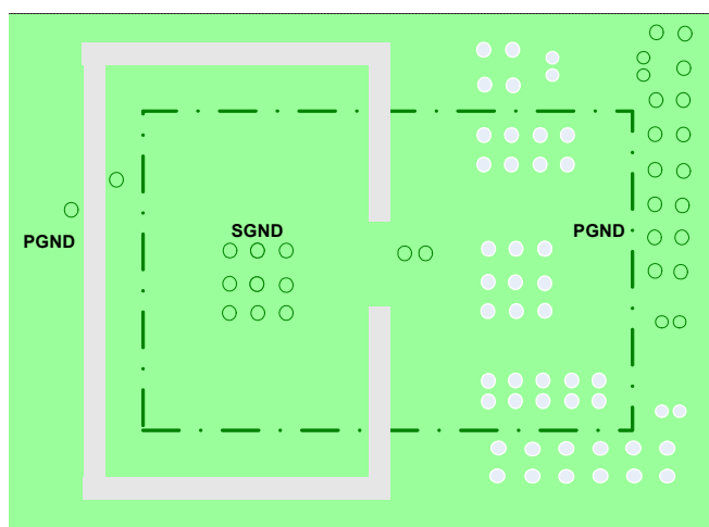
FIGURE 26. RECOMMENDED LAYOUT
