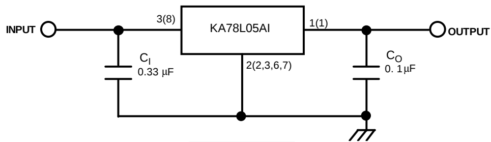
Figure 2. Typical Application
