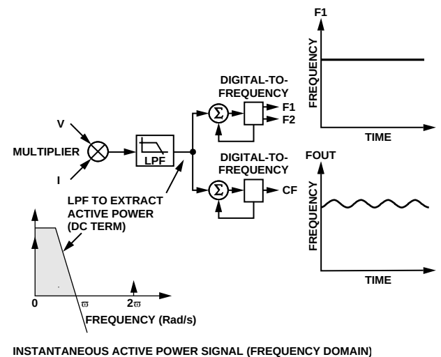
Figure 22. Active Power to Frequency Conversion
