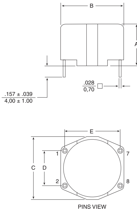
Style 3 - Horizontal Package
