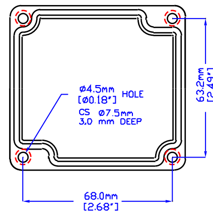
VIEW INSIDE LID
