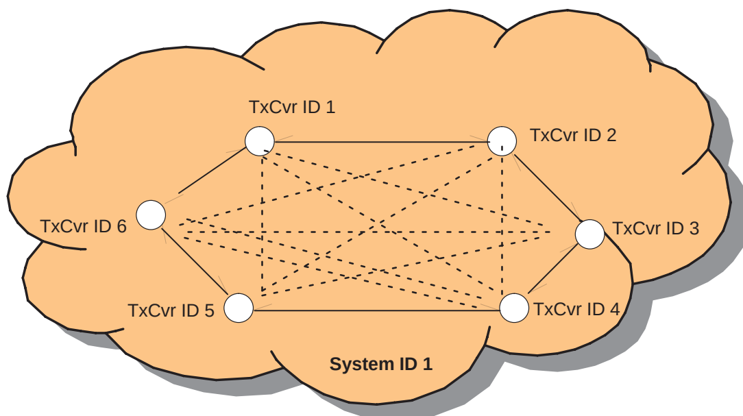
Figure 6-3. Complete Topology
