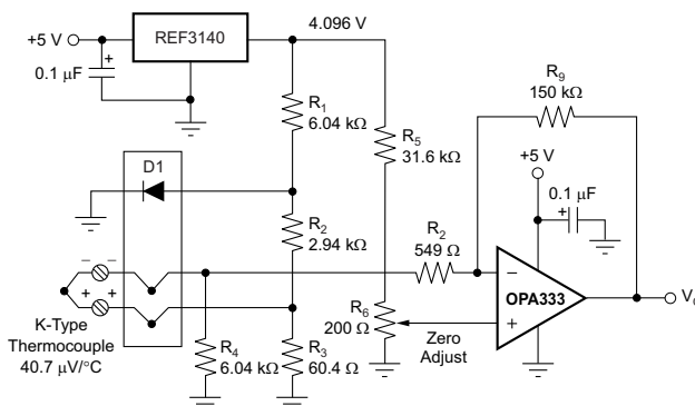
Figure 27. Temperature Measurement
