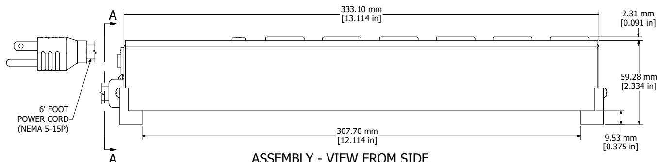
ASSEMBLY - VIEW FROM SIDE
