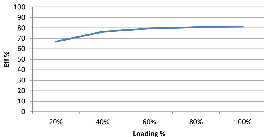
AM1D-0505SZ Efficiency vs. Loading
