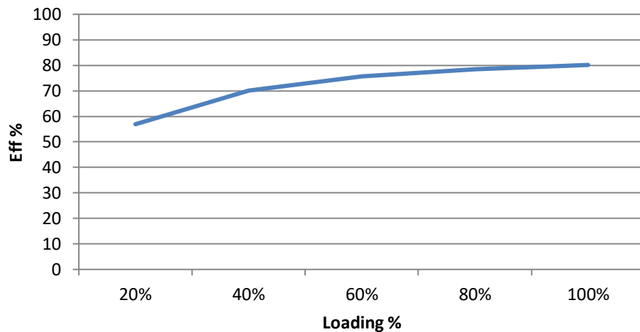
AM1D-1212SZ Efficiency vs. Loading
