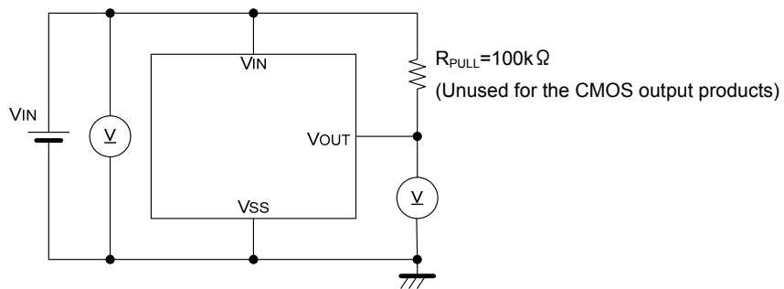
Circuit 1
