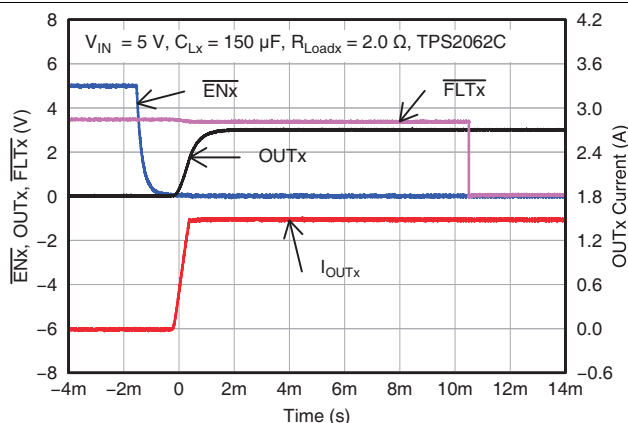
Figure 7. TPS2062C Power Up – Enabled
