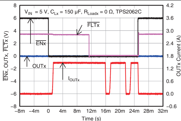
Figure 11. TPS2062C Enable and Disable into Output Short
