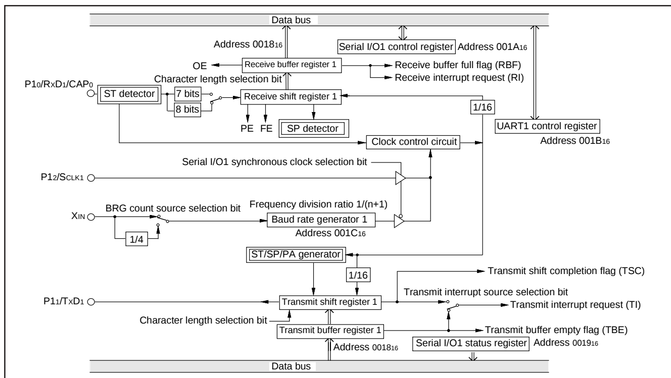
Fig. 54 Block diagram of UART serial I/O1
