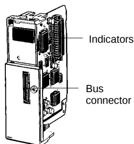
C200HW-COM01
