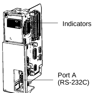
C200HW-COM02
