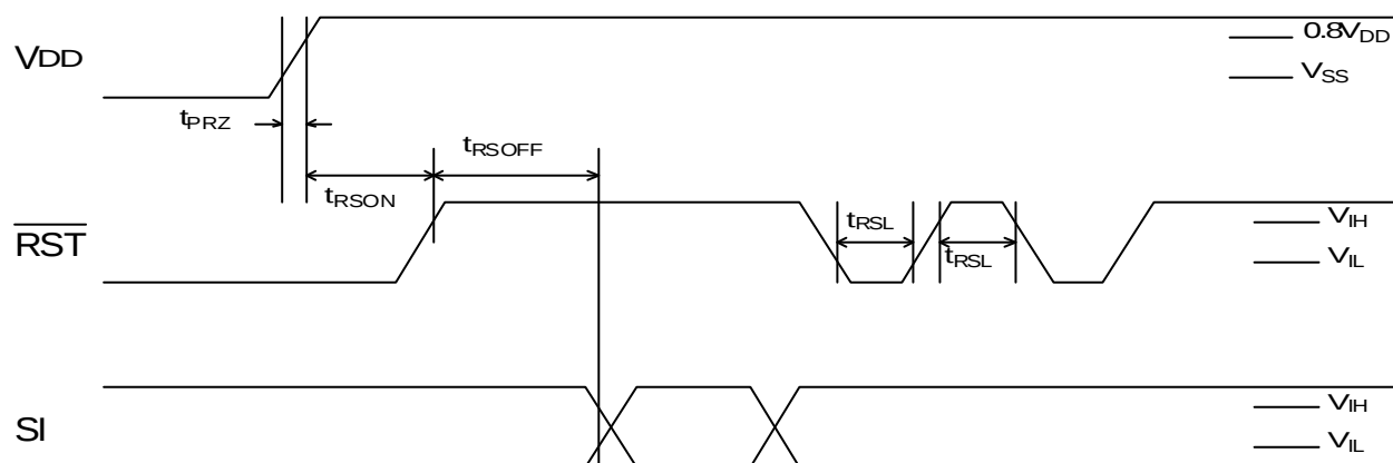
Fig.2 Reset Timing
