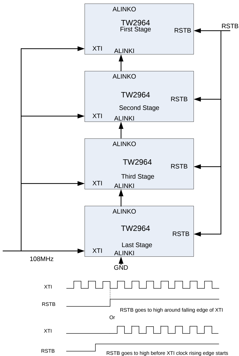
FIGURE 12. RSTB CONTROL FOR 108MHZ XT INPUT
