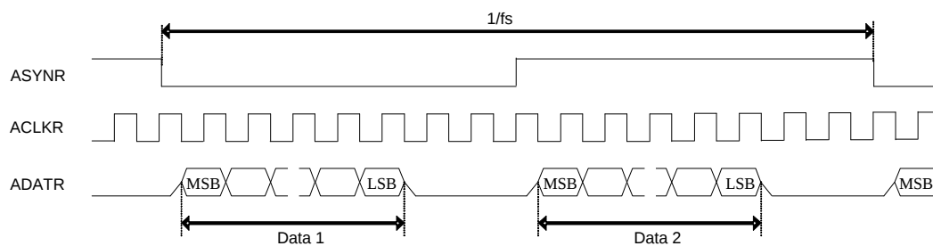
FIGURE 17. ACLKMASTER=0, RM_SYNC=0, ASYNROEN=1
