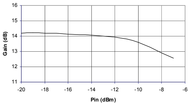
Gain vs. Pin Medium Gain State (10)
