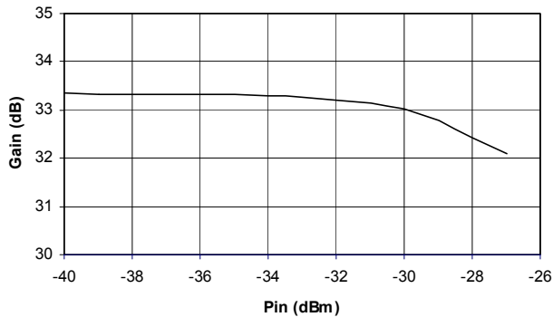
Gain vs. Pin High Gain State (11)
