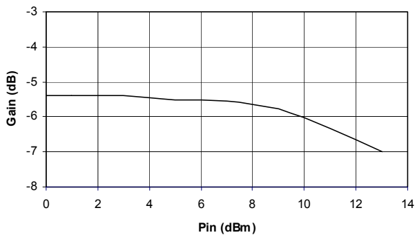
Gain vs. Pin Medium Gain State (10)
