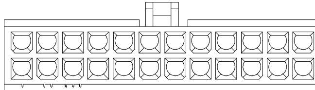
24 POS
