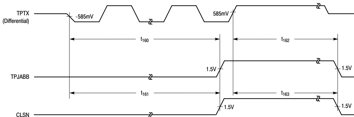
Figure 28. TPJABB Switching
