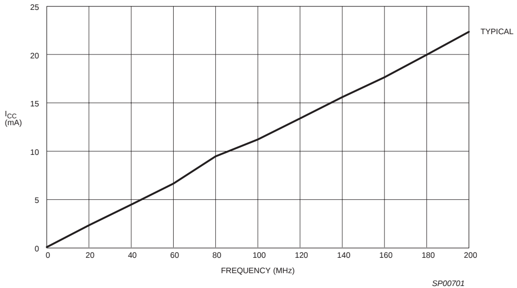
Figure 5: I_{CC} vs. Frequency at V_{CC} = 3.3 V, 25°C
