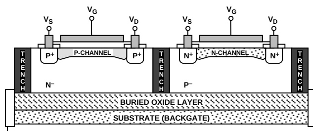
Figure 11. Trench Isolation
