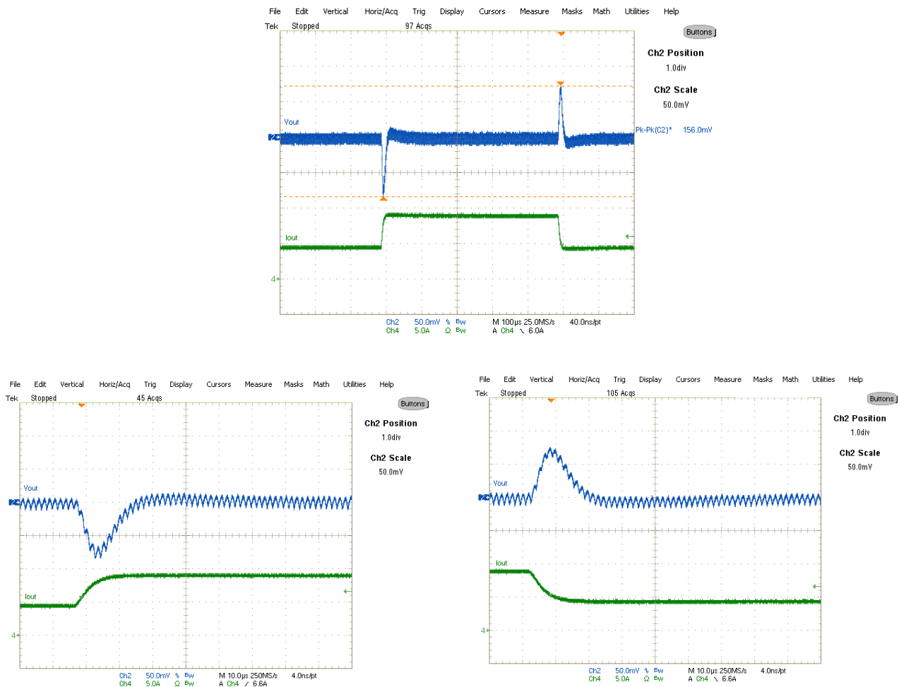
Fig. 24: Transient Response, 4.5A to 9A step 2.5A/ \mu s
