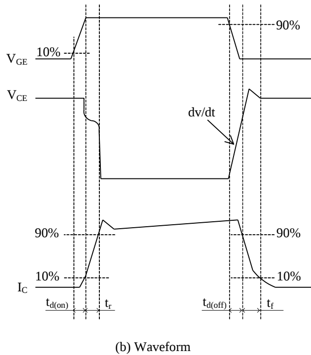
Figure 1 Test Circuits and waveforms of dv/dt and Switching Time
