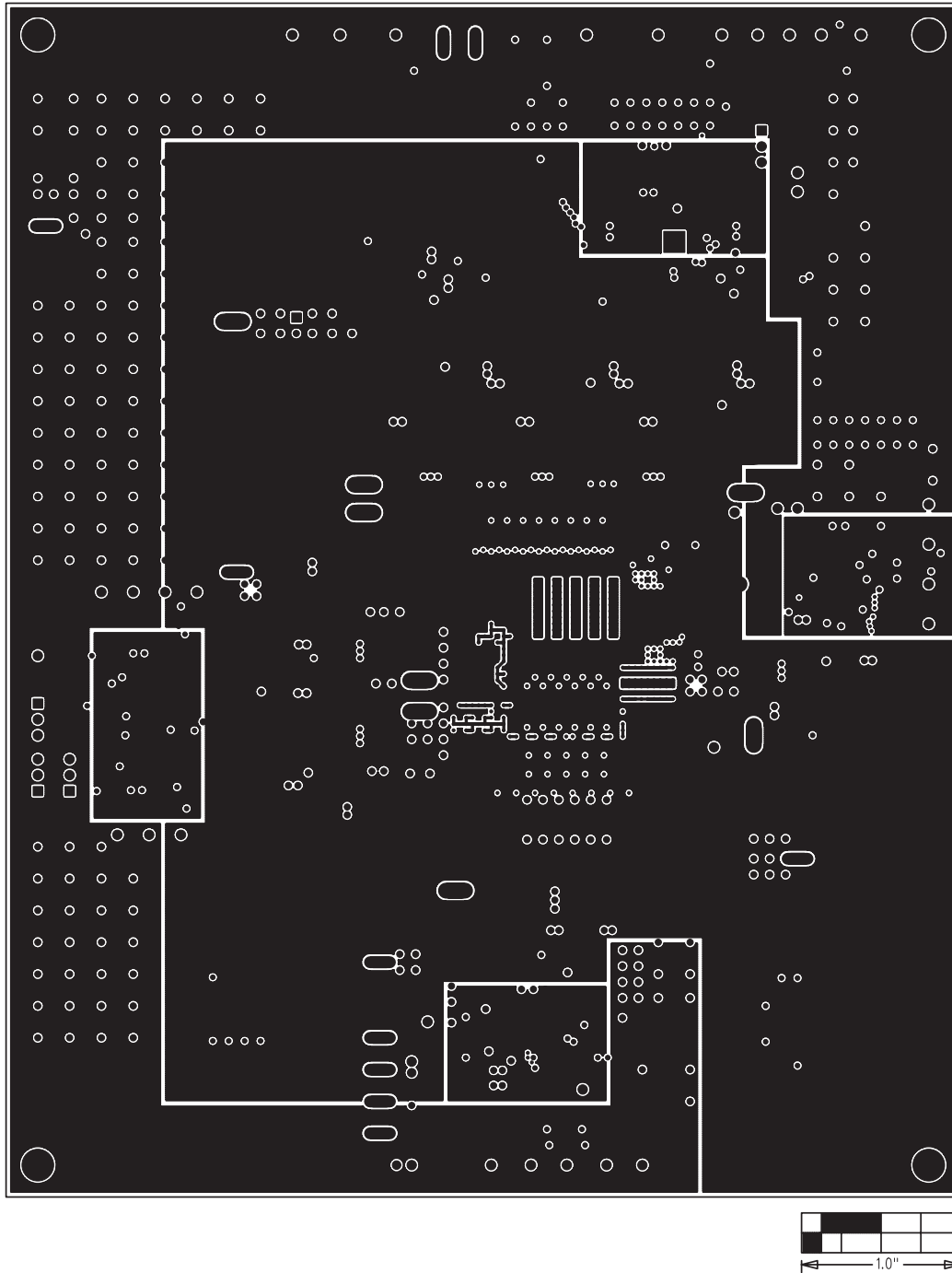
Figure 6. MAX17030 EV Kit PCB Layout—Internal Layer 4 (AGND/PGND Layer)
