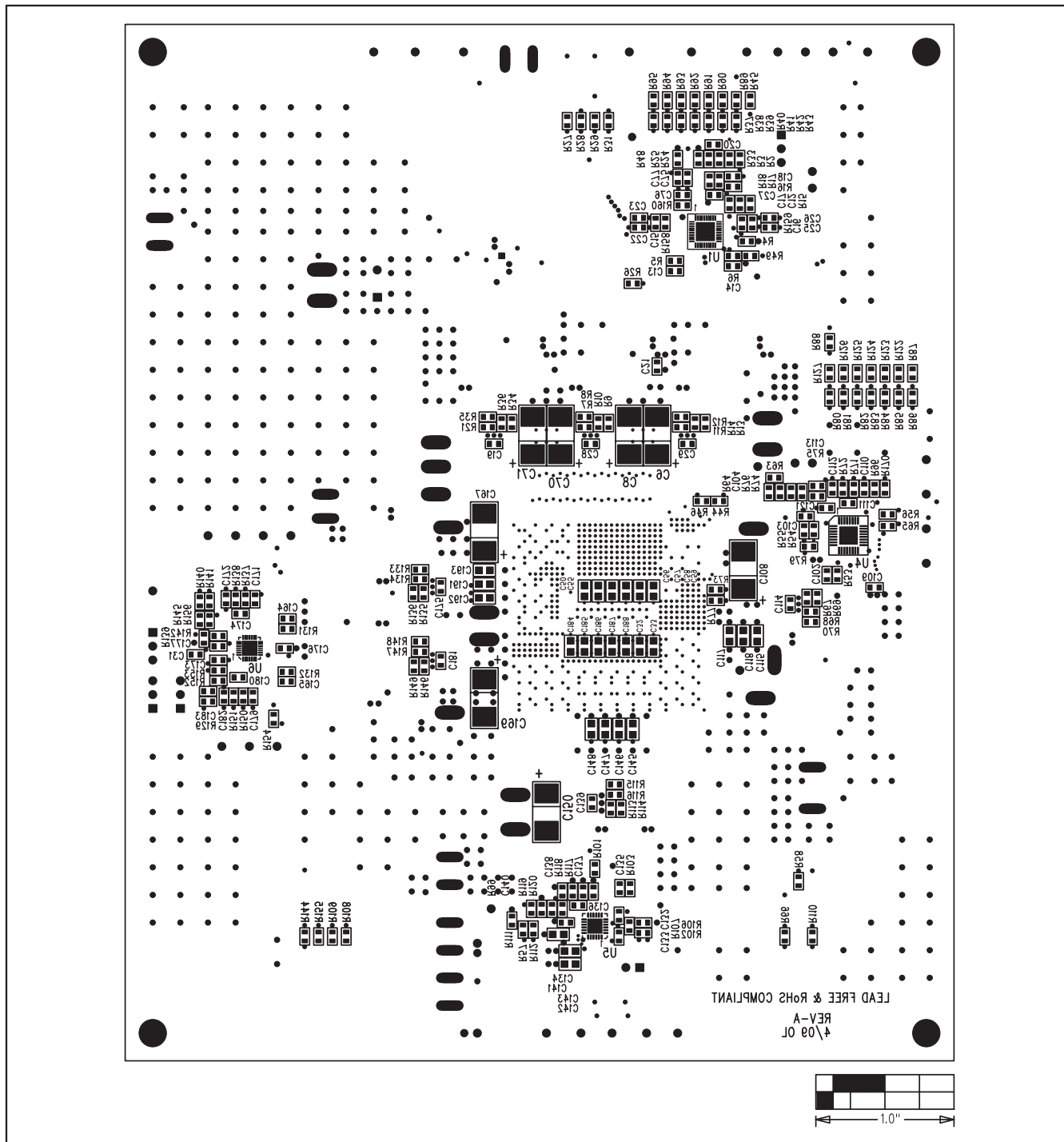
Figure 11. MAX17030 EV Kit Component Placement Guide—Solder Side
