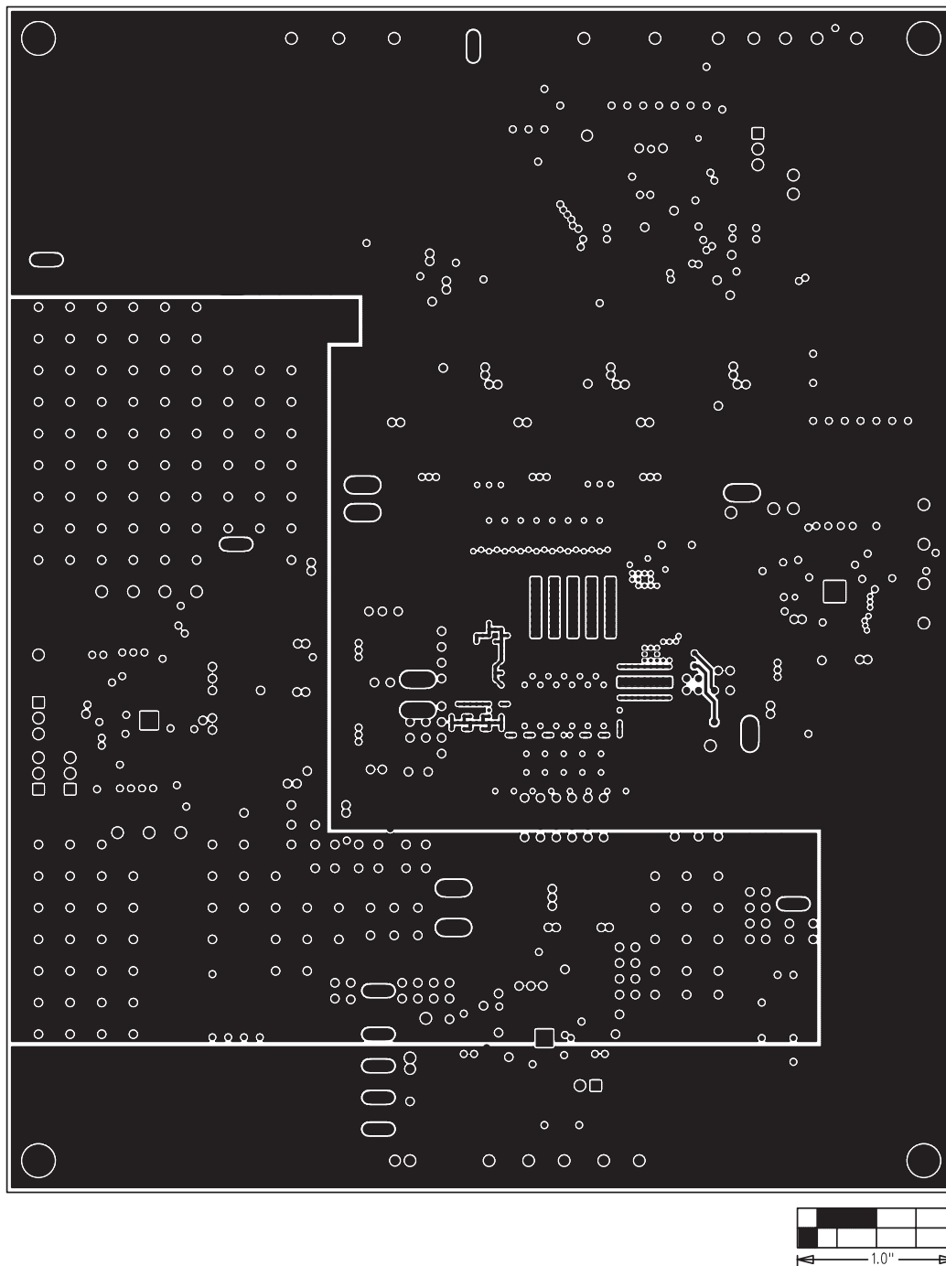
Figure 7. MAX17030 EV Kit PCB Layout —Internal Layer 5 (PGND Layer)
