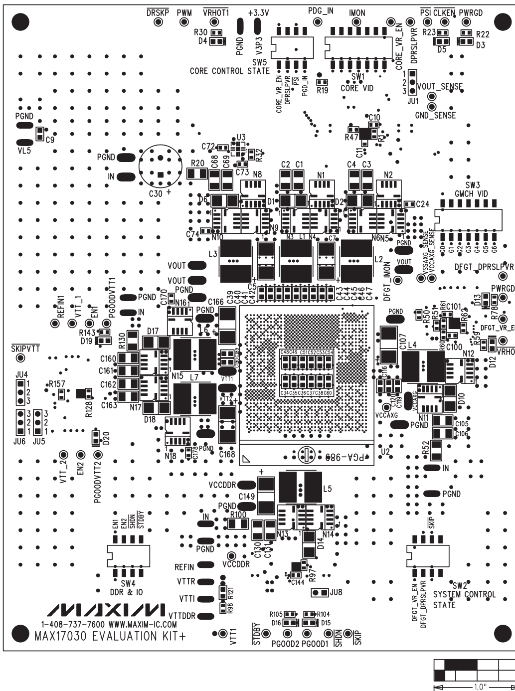
Figure 2. MAX17030 EV Kit Component Placement Guide—Component Side
