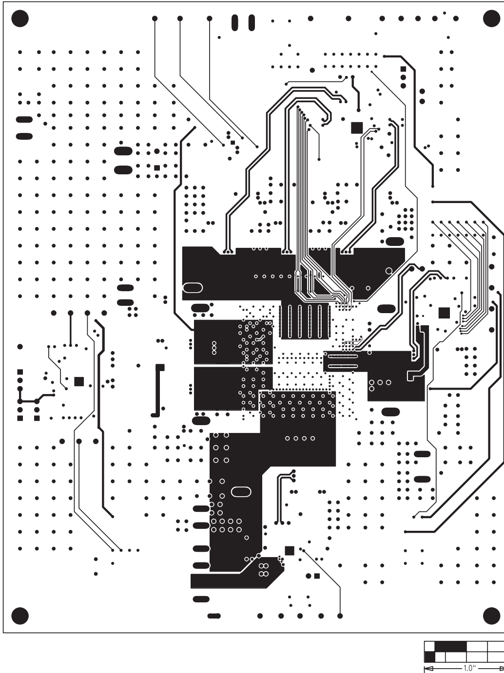
Figure 8. MAX17030 EV Kit PCB Layout —Internal Layer 6 (Signal Layer)
