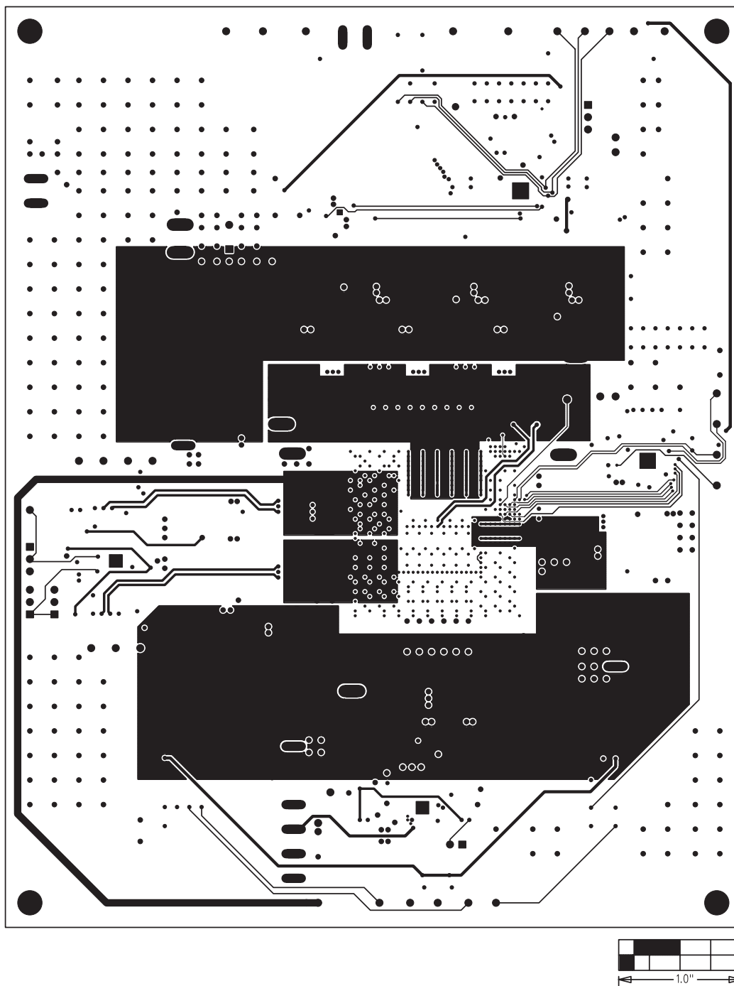
Figure 5. MAX17030 EV Kit PCB Layout—Internal Layer 3 (Signal Layer)
