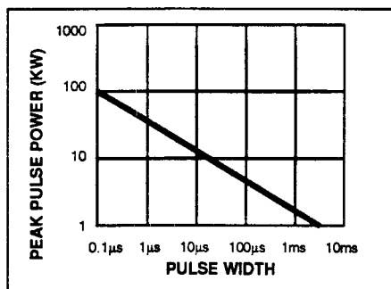
PEAK PULSE POWER VS. PULSE WIDTH
