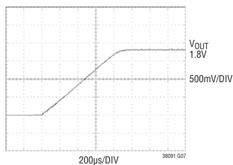
Start-Up with Internal Soft-Start ( \text{TRACK/SS} = V_{IN} )
