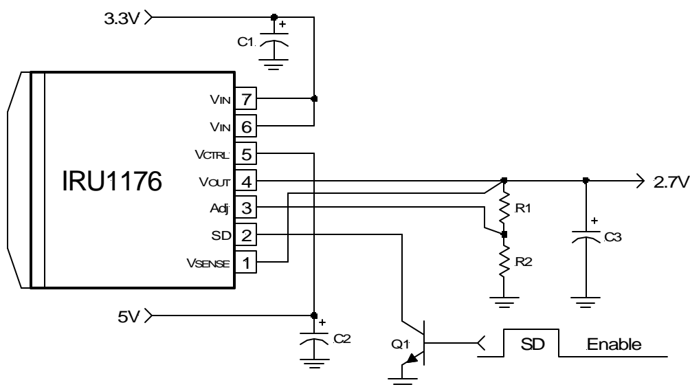
Figure 1 - Typical application of IRU1176.
