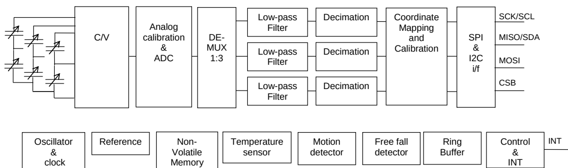
Figure 1. SCA3000 Block Diagram.
