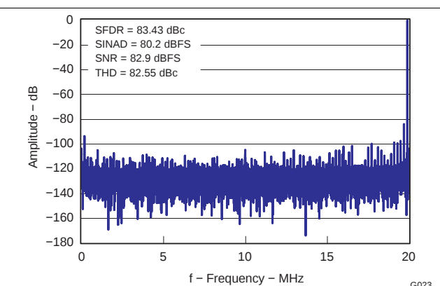
Figure 23. FFT for 20 MHz, –1-dBFS Input Signal
