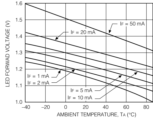
Figure 1. LED Voltage vs. Temperature
