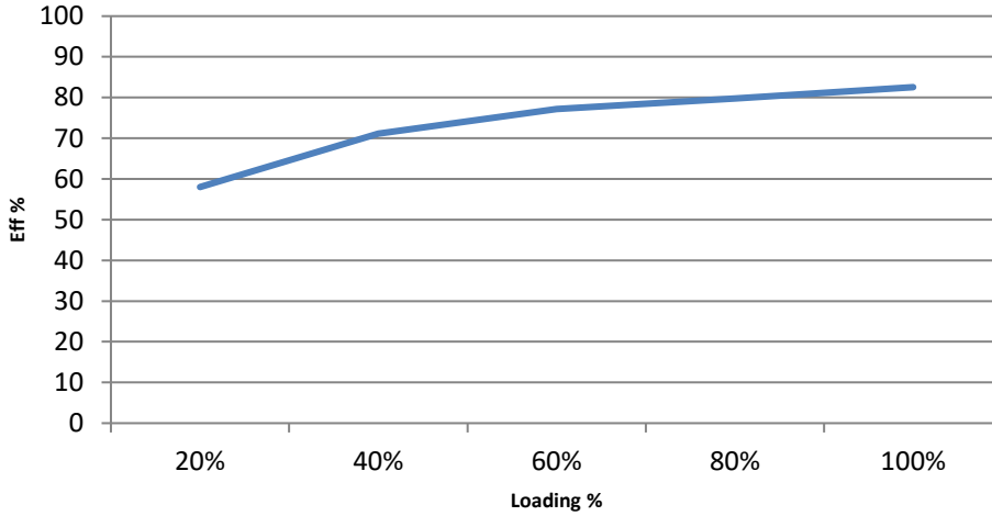
AM1P-2424SZ Efficiency vs. Loading
