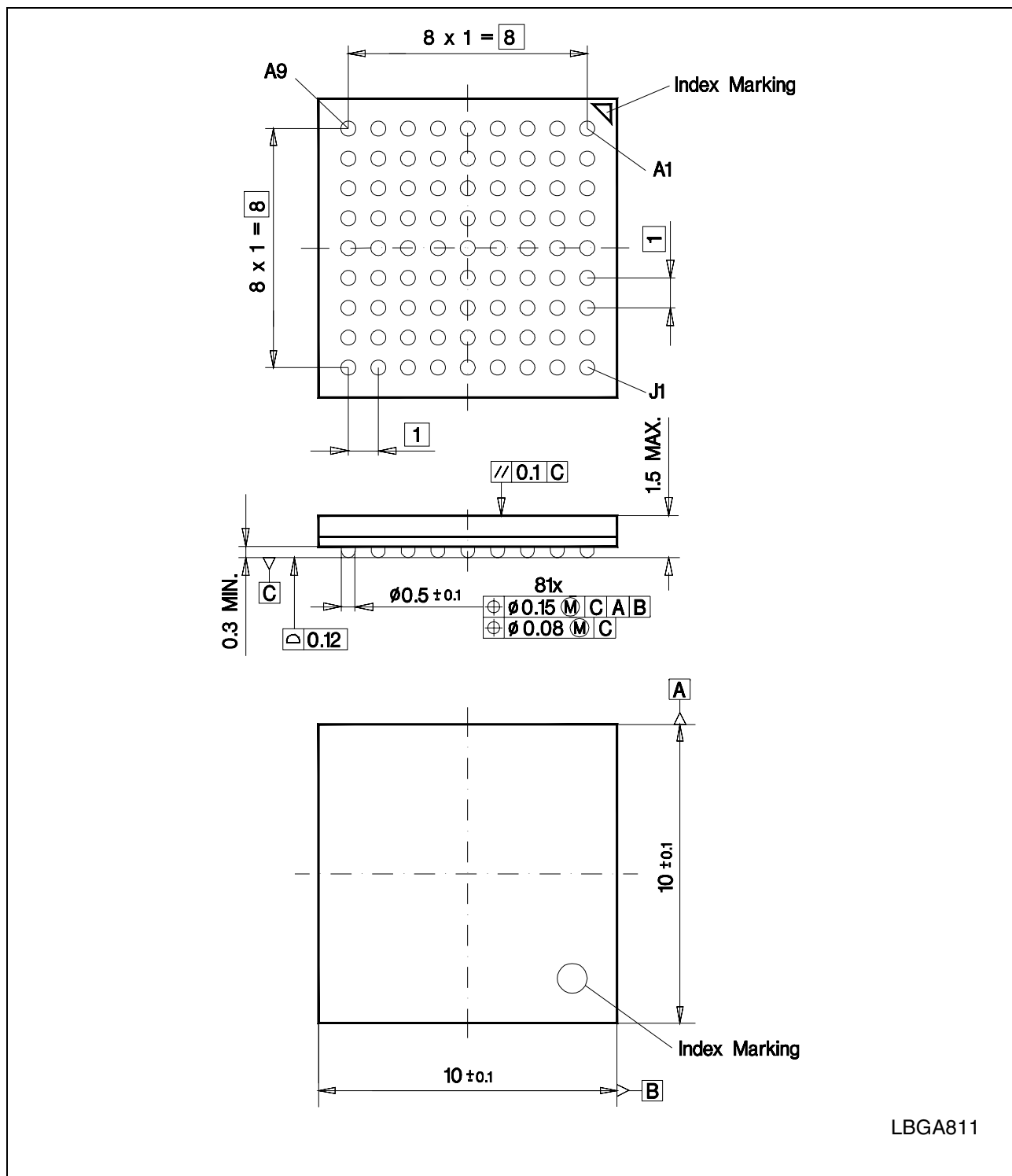
Figure 115 P-LBGA-81-1(Plastic Ball Grid Array Package)
