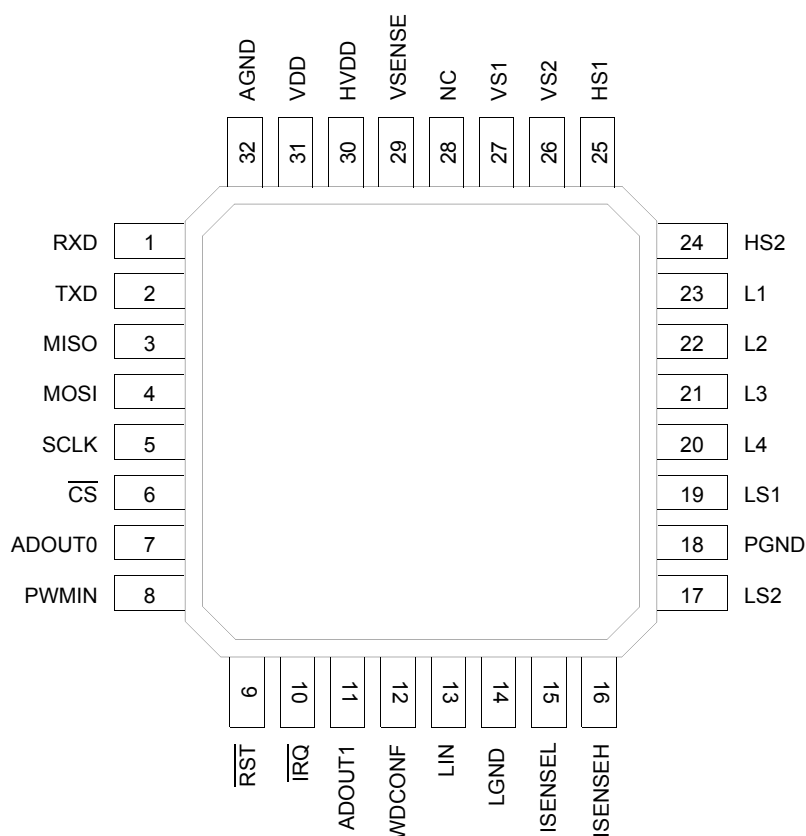
Figure 3. 33912 Pin Connections
