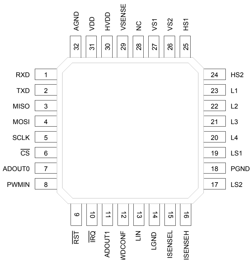
Figure 26. 33912 Pin Connections
