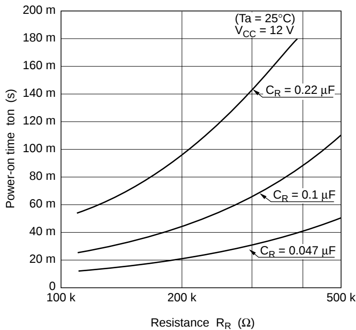
Figure 3 Characteristic of Power-On Reset Circuit
