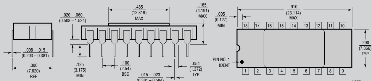
D Package 18-Lead Side Brazed (Hermetic) (Reference LTC DWG # 05-08-1210)
