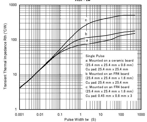
Rth - tw
