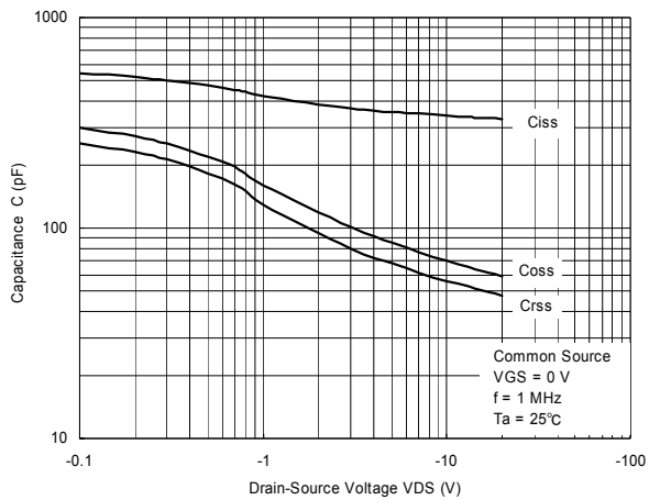
C - VDS
