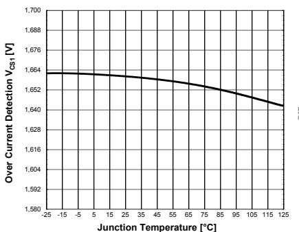
Figure 49 Over Current Detection V_{CS1}
