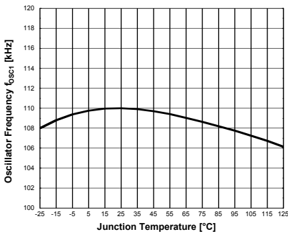
Figure 34 Oscillator Frequency f_{OSC1}
