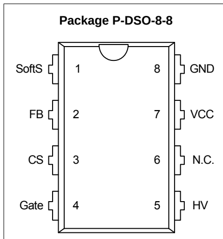
Figure 2 Pin Configuration P-DSO-8-8(top view)
