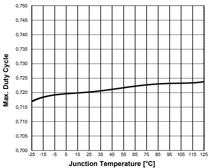
Figure 35 Max. Duty Cycle D_{max}
