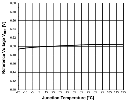
Figure 33 Reference Voltage V_{REF}
