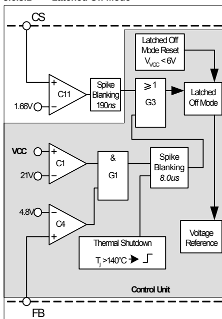
Figure 18 Latched Off Mode
