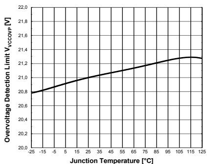
Figure 46 Overvoltage Detection Limit V_{VCCOVF}
