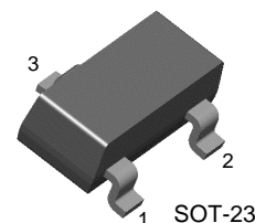
1. Base 2. Emitter 3. Collector SOT-23
