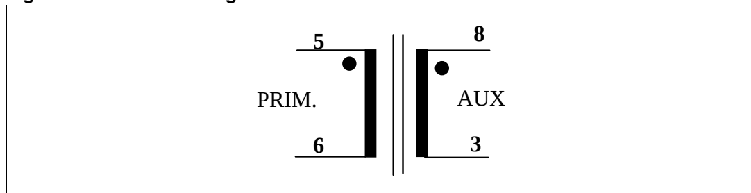
Figure 31. Electrical diagram
