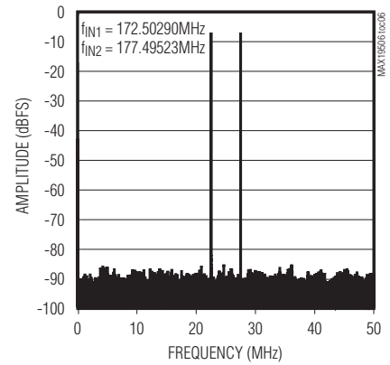
175MHz TWO-TONE FFT PLOT
