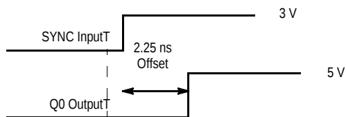
Figure 3. Depiction of the Fixed SYNC to Q0 Offset ( t_{PD} ) Which Is Present When a 470 K \Omega Resistor Is Tied to V CC or Ground
