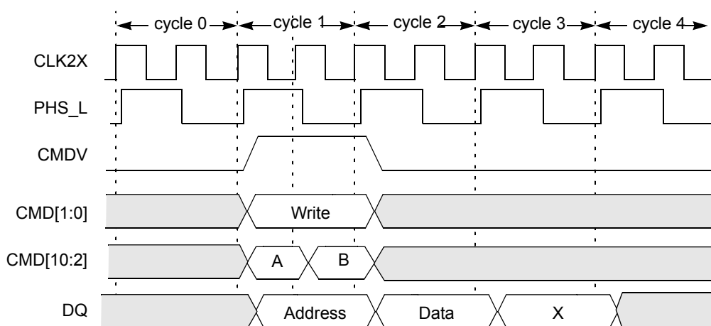
Figure 10-3. Single Write Cycle Timing
