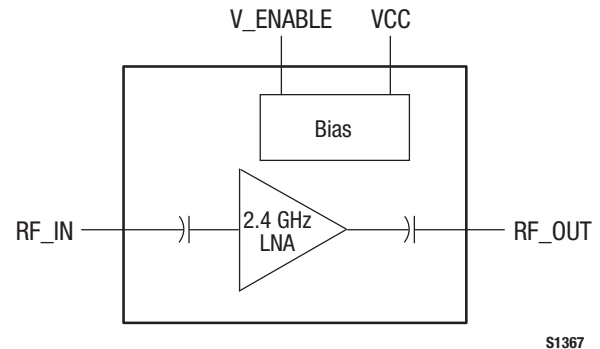
Figure 1. SKY65405 LNA Block Diagram
